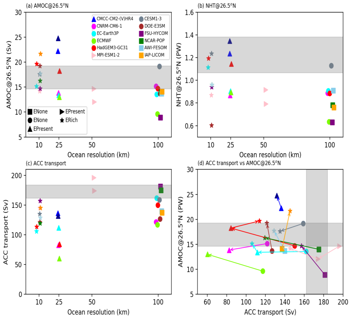
Figure 1: Comparison of multi-model large-scale ocean metrics with observations. (a) AMOC and (b) Northward Heat Transport (NHT) in the Atlantic at 26.5°N; (c) ACC transport (Sv); (d) an illustration of the impact of ocean model resolution on the ACC-AMOC simulation. Model simulations are from CMIP6 OMIP experiments [25] and from CMIP6 HighResMIP control-1950 experiments [73] (plus additional data not yet archived, see Model Data for details). AMOC/NHT observations [66, 67] are shaded with the annual mean range between 2004-2017. ACC observations from the cDrake array [83] are shaded indicating 173 \pm 11 Sv.
