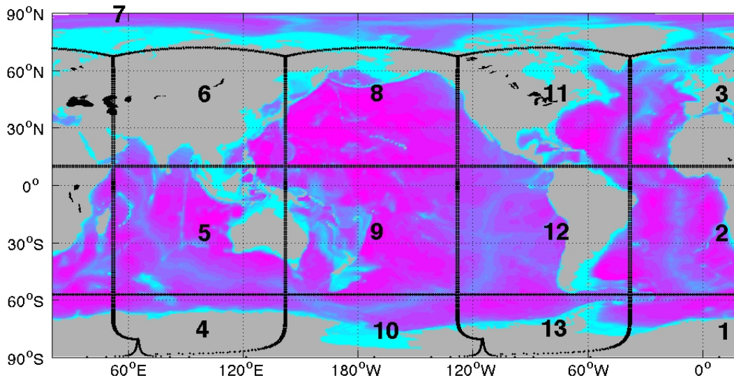
Figure 1: ECCOV4 tiles the Earth.
