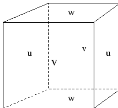
Figure 2: MITgcm gridcell with velocity component’s central location labeled.
