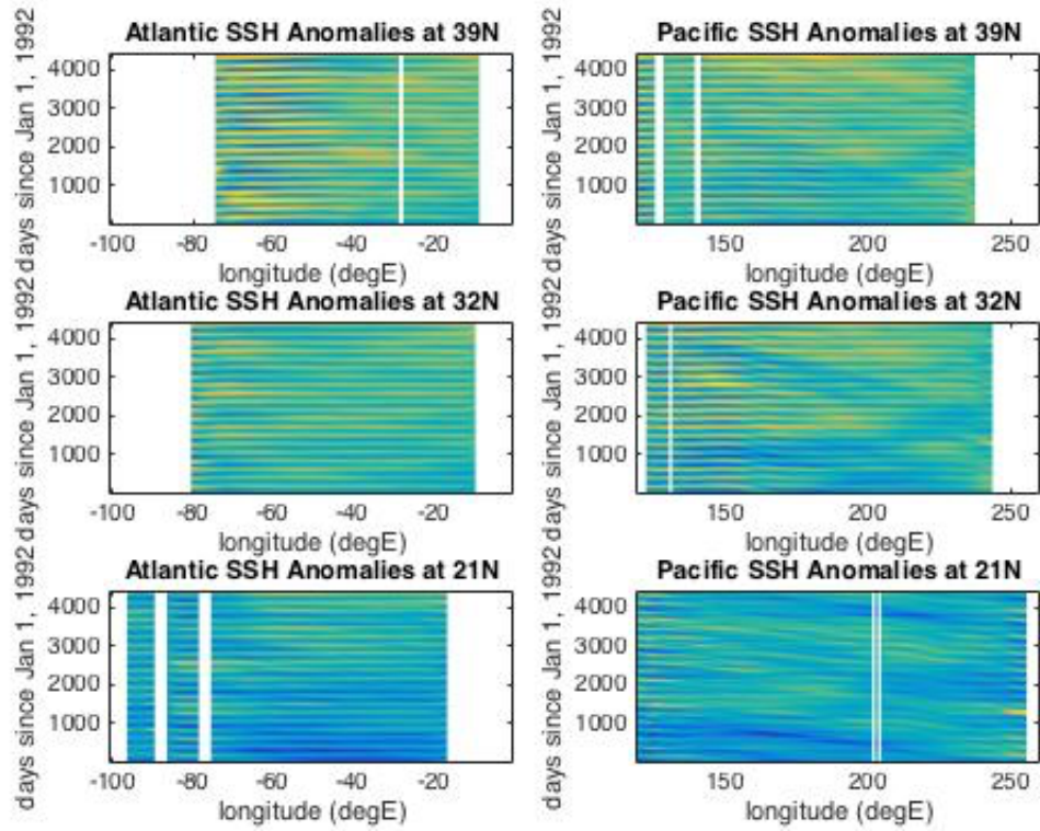
Figure 2: Hovmuller diagrams of SSH.
